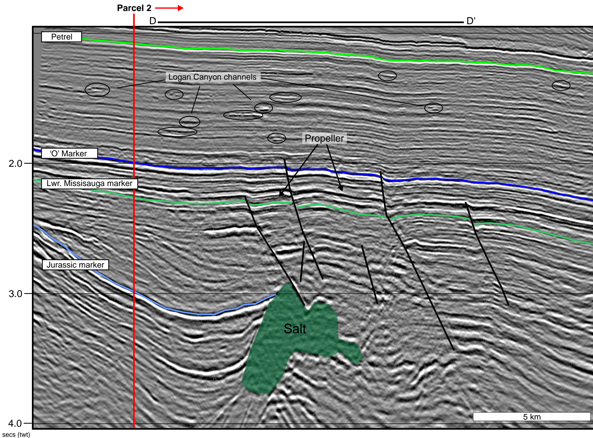
Seismic profile D-D' through the Propeller prospect. Some younger Logan Canyon channels are also identified on this profile. The northern boundary of Parcel 2 is represented by the red line on the left side of the figure.
